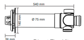
Direct Flue Kit LSDFK01
